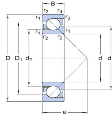
7310,Single Row Angular Contact Ball Bearing
